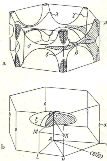
Fig. 1. The Fermi surface of zinc according to Gibbons and Falicov. a) First and second band of holes (first band "caps" are shown crosshatched). b) Third band of electrons. The capital letters designate symmetry points of the Brillouin zone and the small greek letters show the orbits discussed in the text
